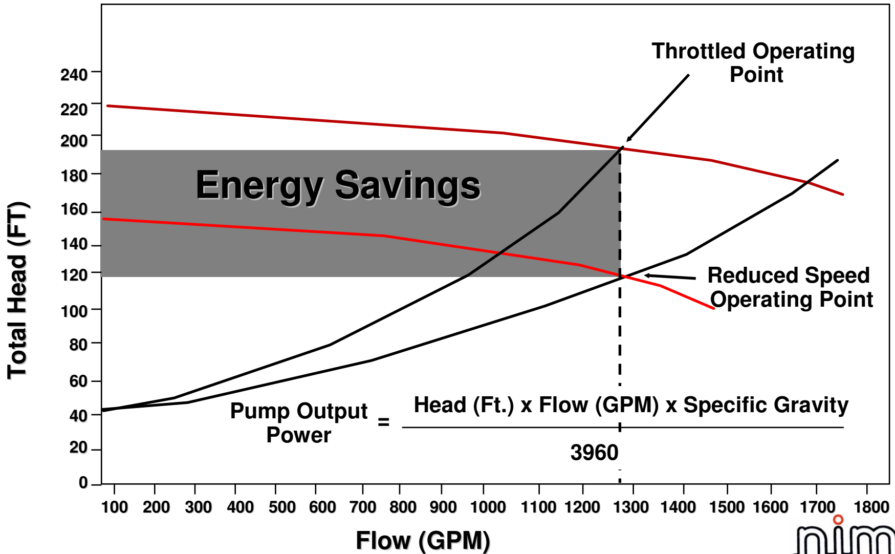
80% Flow, 1280 GPM Valve Operation Versus Reduced Speed Operation
